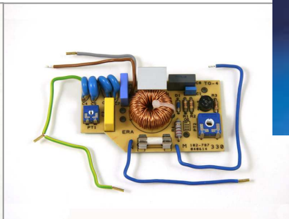
Motor Speed Controller 500 W
