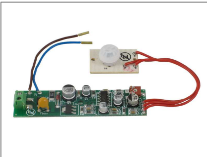
Fan Motor Timer and Control Unit with PIR Sensor
