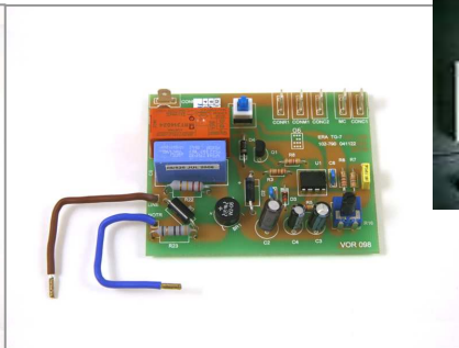
Manuel Hand Dryer Control Unit
