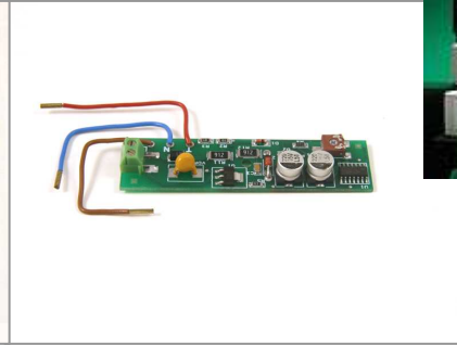
SMD Fan Timer and Motor Control Unit
