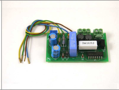
Fan Timer Motor (2 Speed) Control Unit (SMD & Leaded Components)
